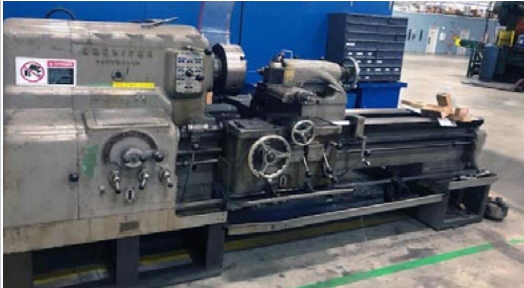
AMERICAN 20" x 54" Engine Lathe
