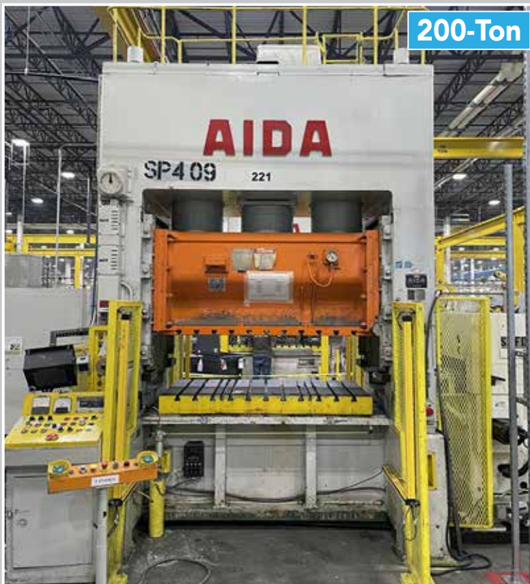
200-TON AIDA PDA-20M SS Press
